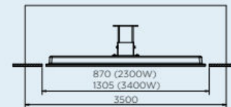
MINIMUM CAVITY OPTION 2 2300/3400W
