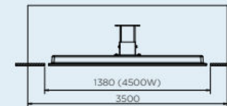
MINIMUM CAVITY FOR 4500W
