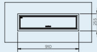
CEILING RECESS FRAME 2300W
